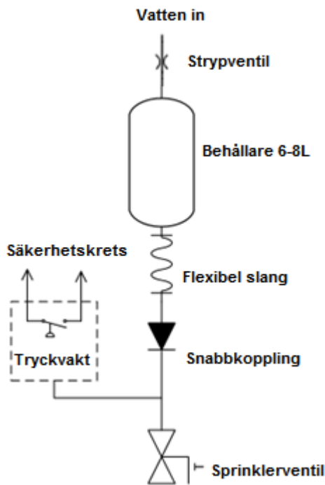
Figur 8 Sprinkler installation
