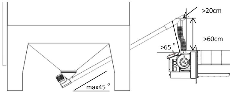
Figur 9 Extern skruv installation
