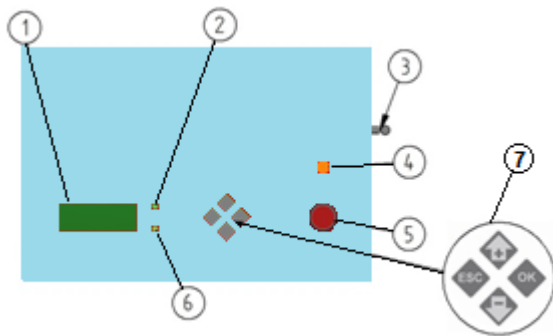
Figur 16 Kontrollpanel
