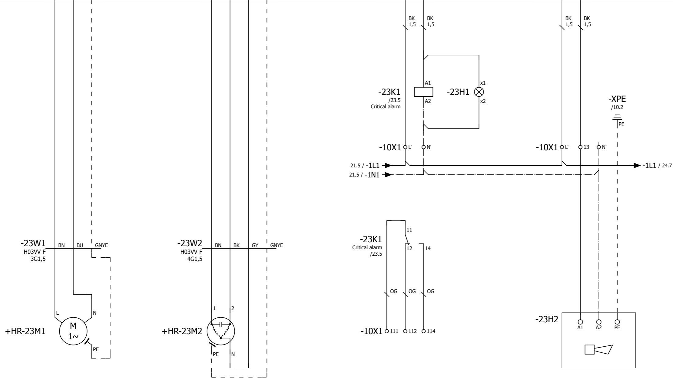
Bypass pump
