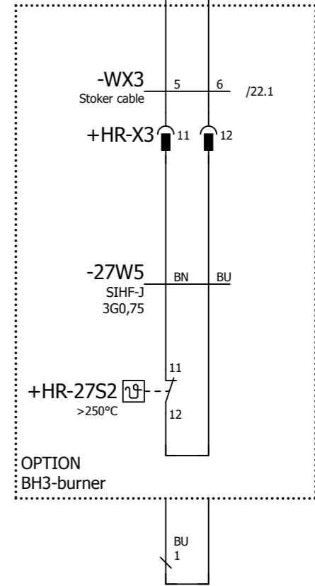
Terminal thermal overload Klixon
