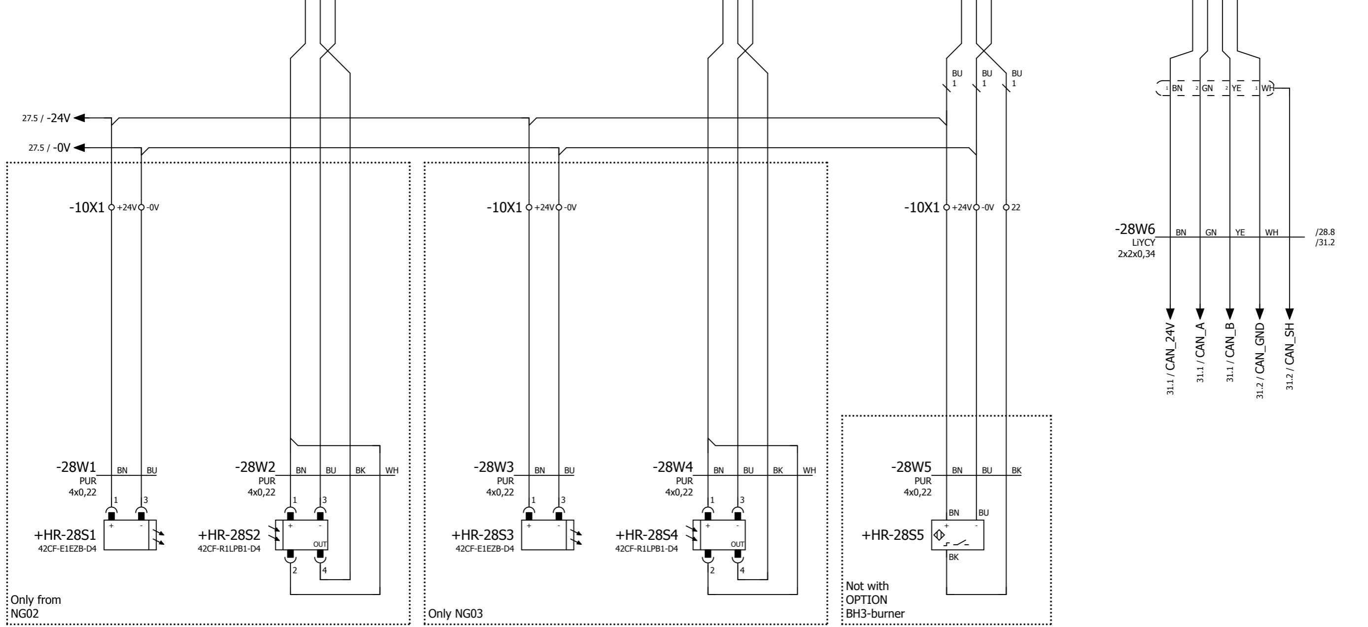
Light sensor transmitter auger 1
