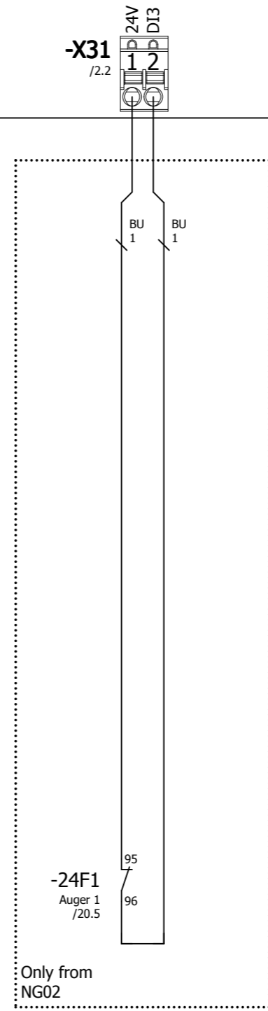
Boiler door High limit stat External enable Terminal thermal overload fuel auger 1 Terminal thermal overload stoker auger Terminal thermal overload ash discharge
