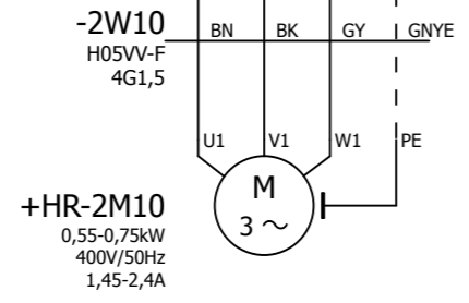
Stokerauger forward
