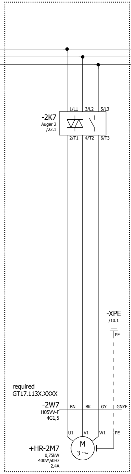
Auger 2
